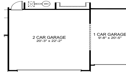
Opt 3rd Car Garage
