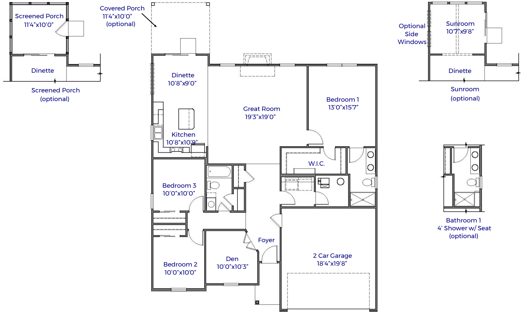
FIRST FLOOR
