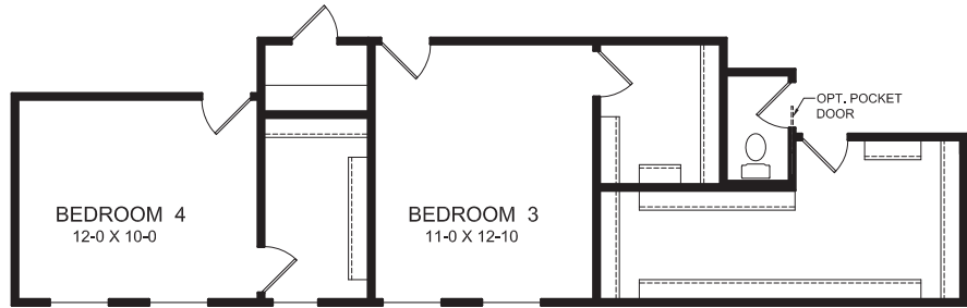
INCLUDED SECOND FLOOR w/ OPT. FIRST FLOOR LAUNDRY
