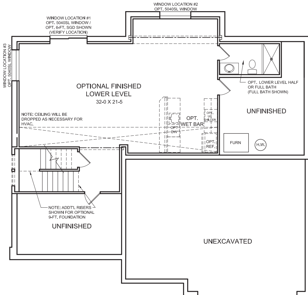
OPTIONAL FINISHED LOWER LEVEL DESIGN INCLUDED 8-FT BASEMENT CLG. HEIGHT
