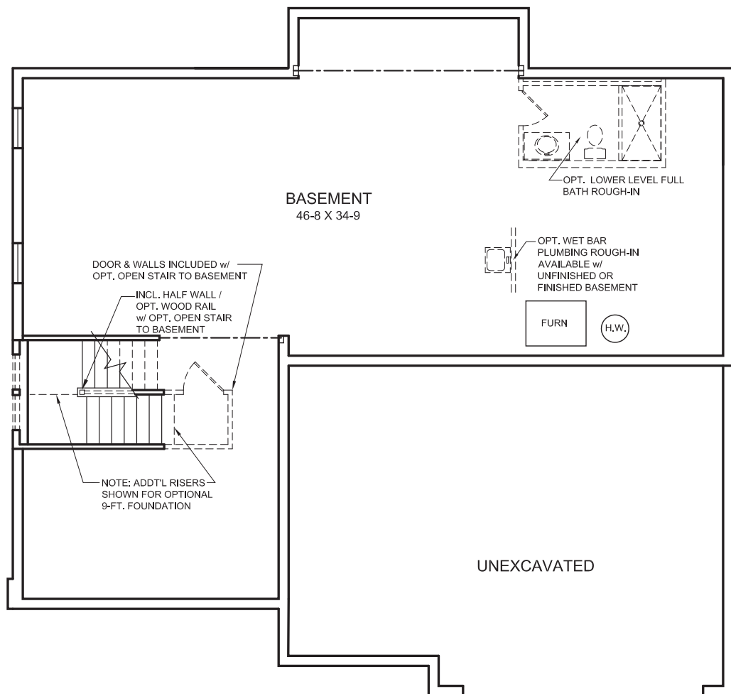
BASEMENT DESIGN INCLUDED 8-FT BASEMENT CLG. HEIGHT
