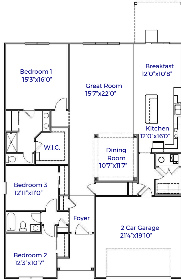
Covered Porch 12'0" x 10'0" (optional)
