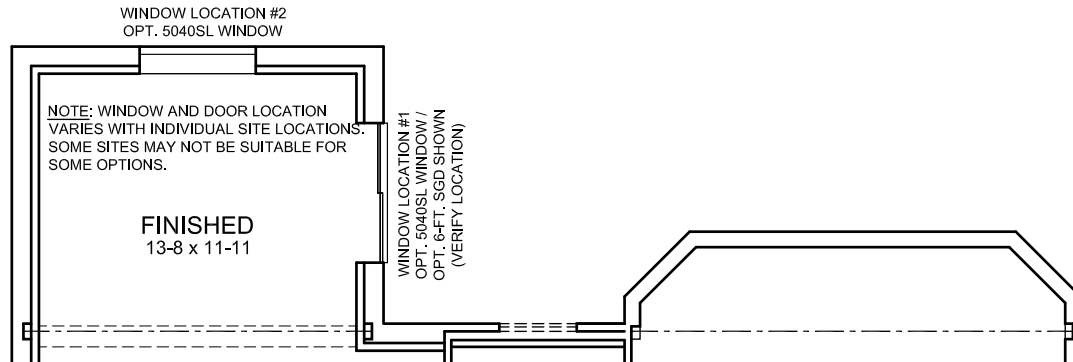
OPTIONAL FINISHED LOWER LEVEL DESIGN w/ OPT. SUNROOM
