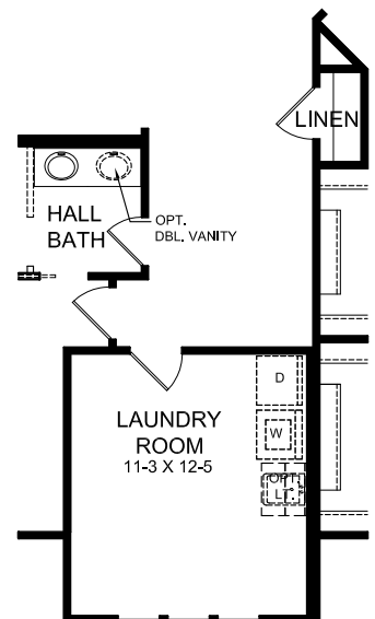
OPTIONAL SECOND FLOOR LAUNDRY FRENCH MANOR EXTERIOR
