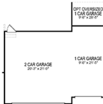
Opt 3rd Car Garage
