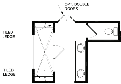
OPTIONAL LUXURY SHOWER
