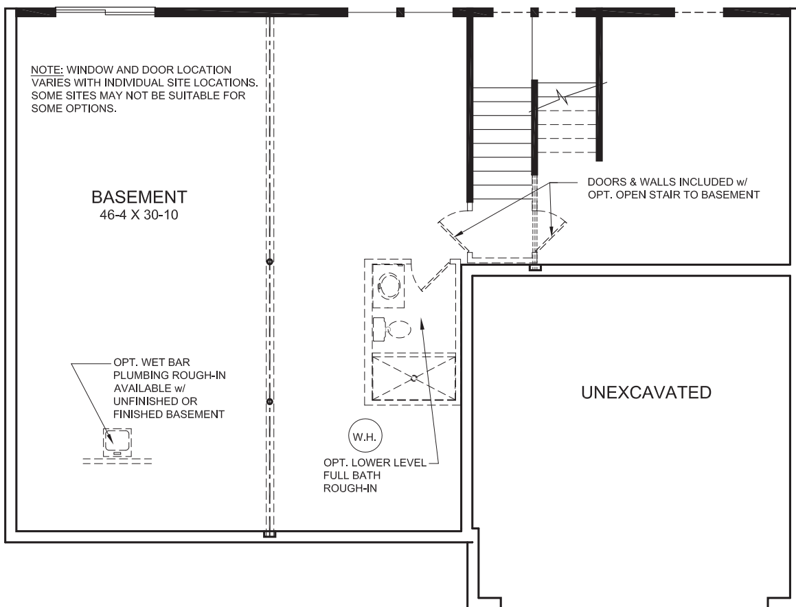
OPTIONAL WALKOUT BASEMENT
