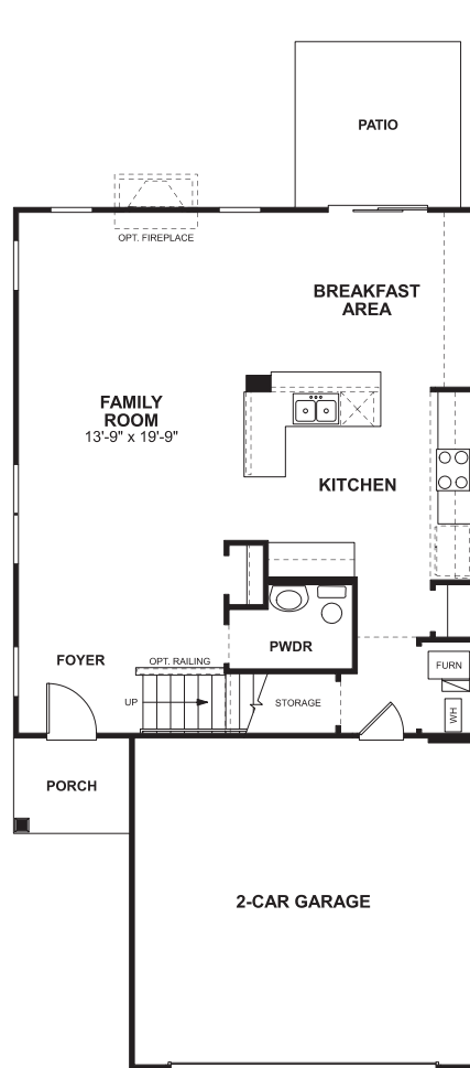
FIRST FLOOR 9' CEILING
