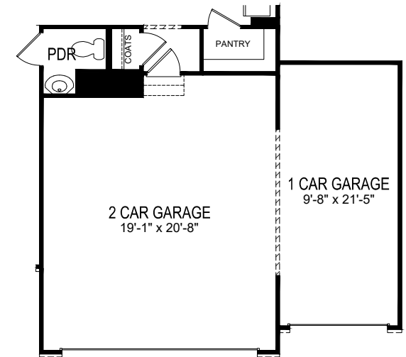
Opt 3rd Car Garage
