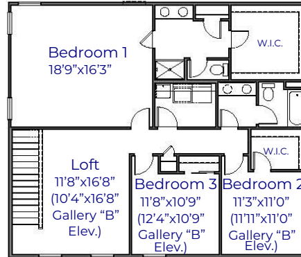
3 Bedroom Second Floor Plan (optional)
