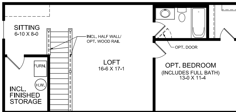
OPTIONAL LOFT DESIGN w/ OPTIONAL BEDROOM & FULL BATH (LOFT NOT AVAILABLE w/ OPT. BASEMENT)
