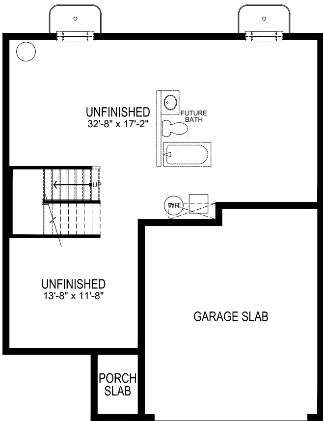
Opt Unfinished Basement
