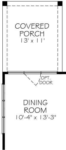
OPTIONAL COVERED PORCH (OFF DINING ROOM)
